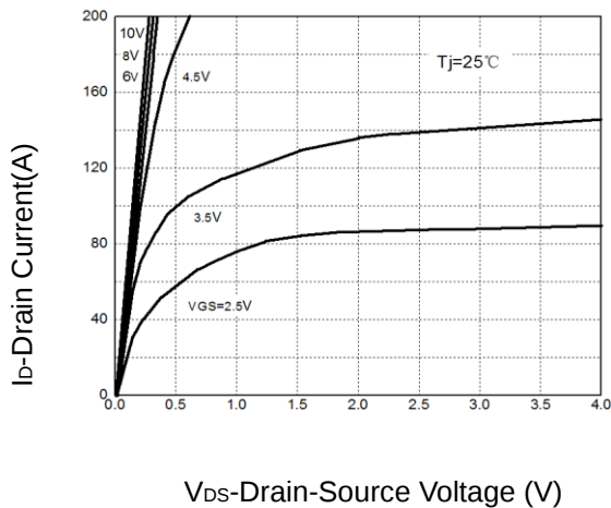
Figure 5: Output Characteristics
