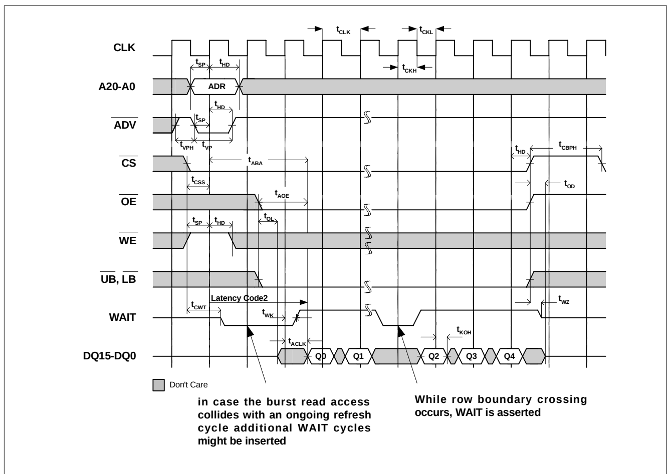
Figure 20 Synchronous Read Burst
