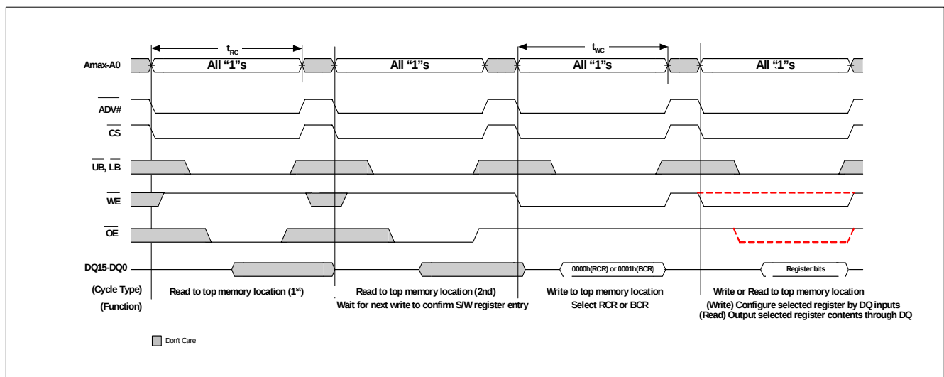
Figure 32 S/W Register Entry timing (Address input = 1FFFh)
