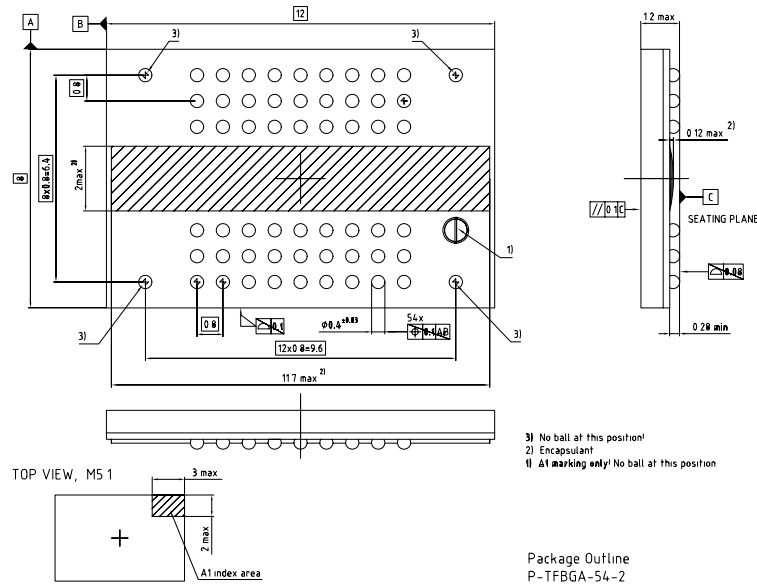
Figure 7 Package Outline TFBGA-54
