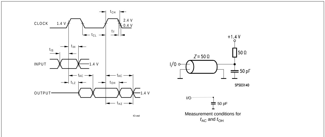
Figure 5 Measurement conditions for t_{AC} and t_{OH}
