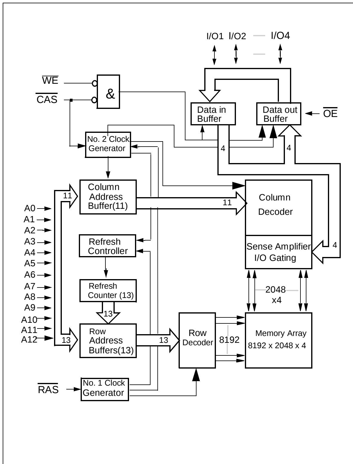
Block Diagram for HYB 3164405AJ/AT(L)
