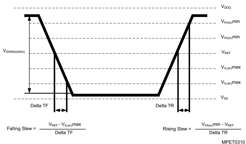
FIGURE 3 Single-ended AC Input Test Conditions Diagram
