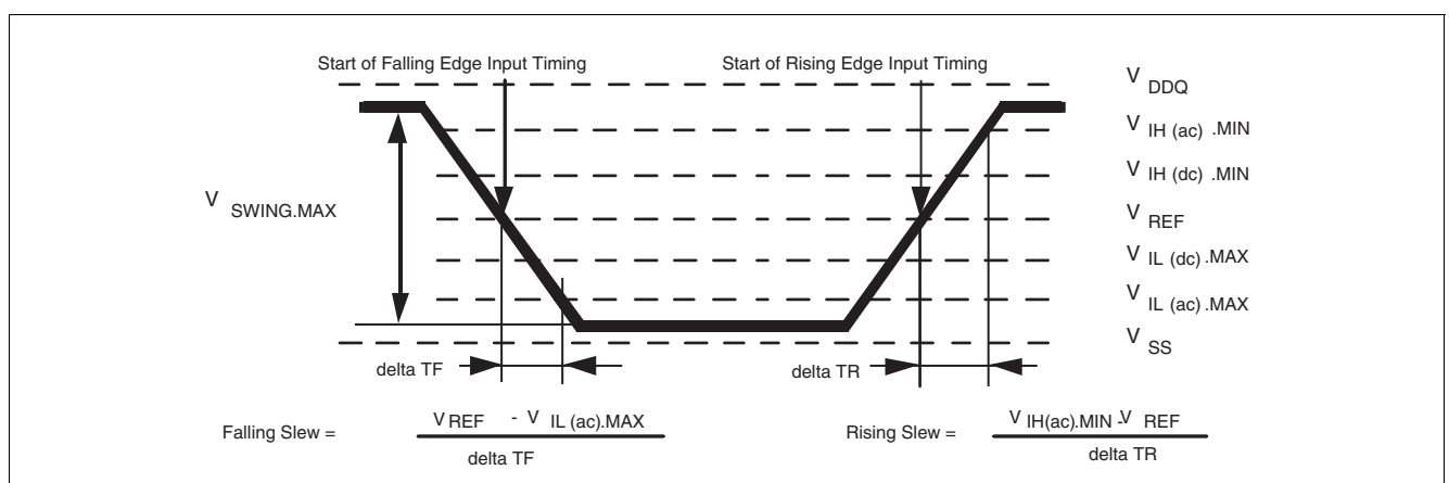
Figure 64 Single-ended AC Input Test Conditions Diagram
