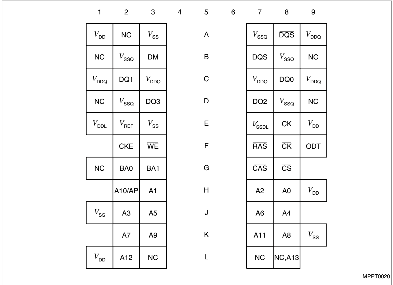
Figure 1 Pin Configuration for ×4 components, P-TFBGA-60 (top view)
