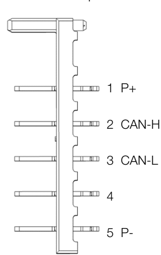
Device Counterpart for CAN-Bus
