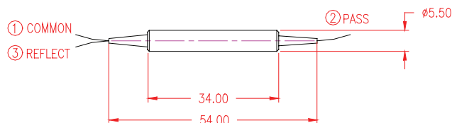
P1: SMF-28 250 \mu m bare fiber
