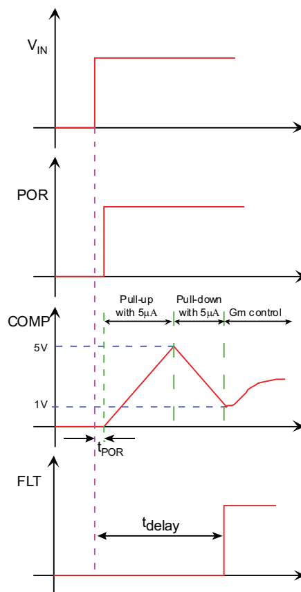
Fig. 2 Waveforms During Startup
