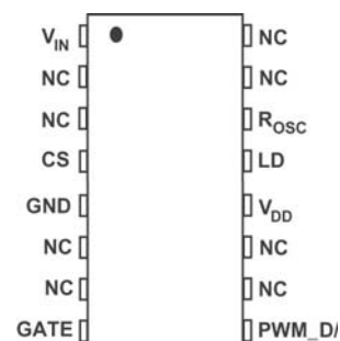
16-Pin SOIC
