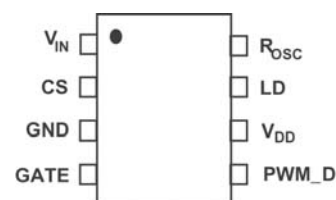
8-Pin DIP/SOIC
