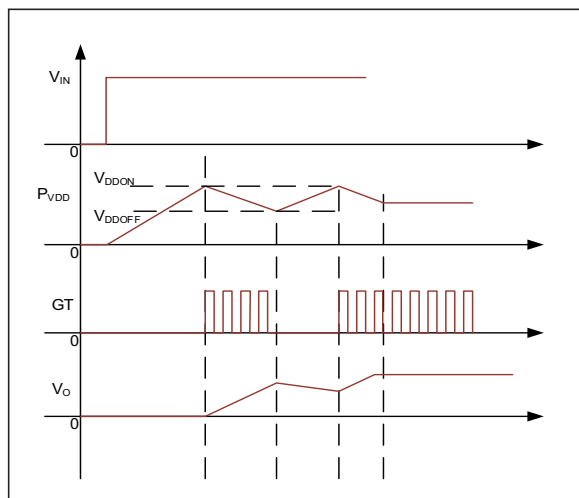
FIGURE 5-1: Typical Startup Waveforms.
