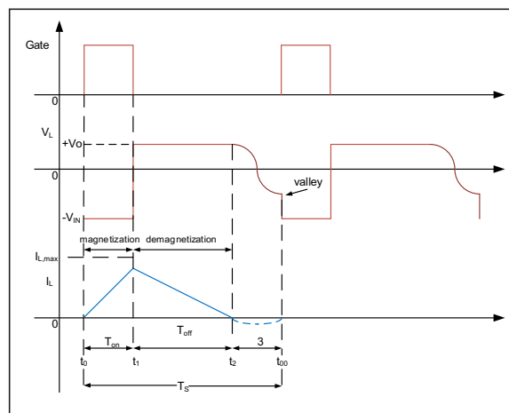
FIGURE 5-2: Valley Detect Waveforms.
