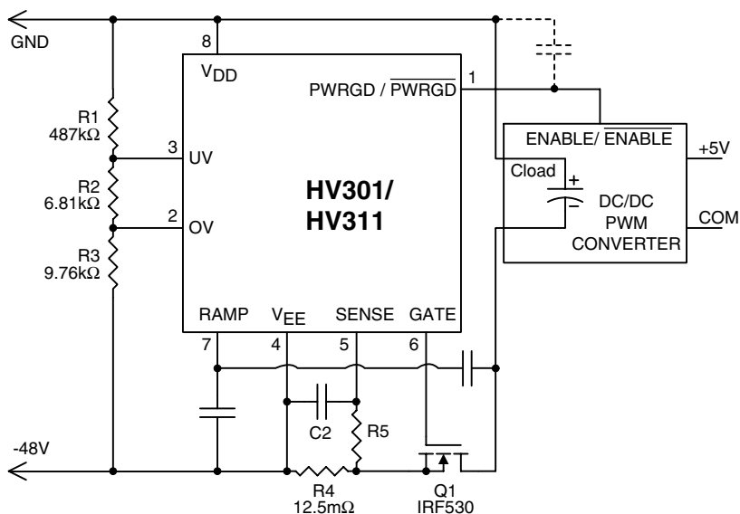
Application Circuit 15
