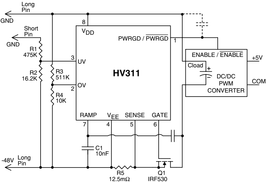
Application Circuit 8
