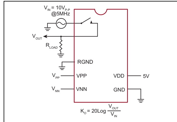
FIGURE 3-4: Off Isolation.
