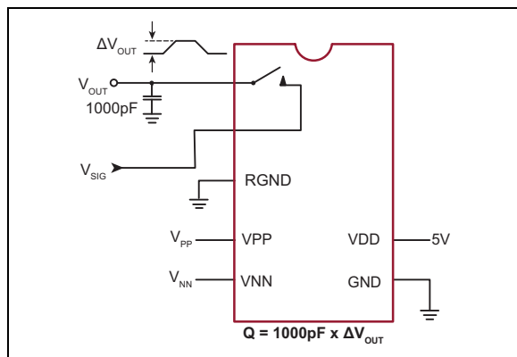
FIGURE 3-7: Charge Injection.
