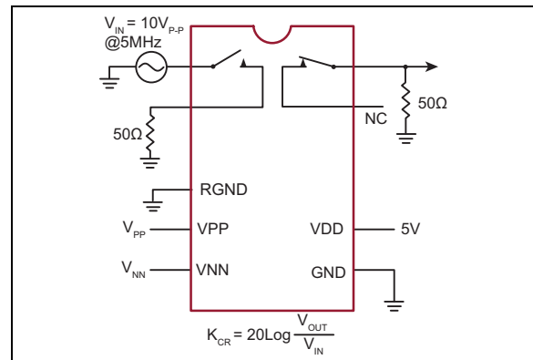
FIGURE 3-6: Switch Crosstalk.
