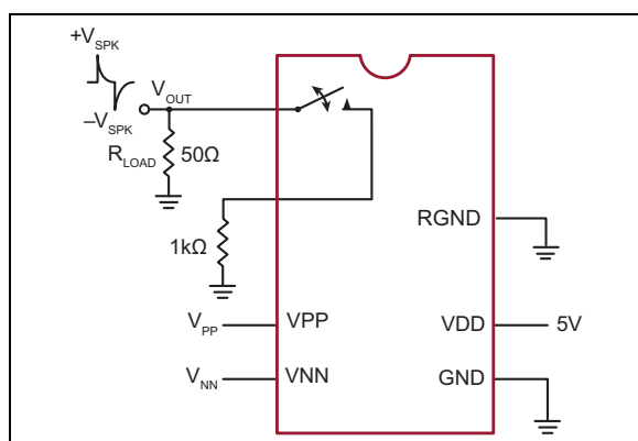
FIGURE 3-8: Output Voltage Spike.
