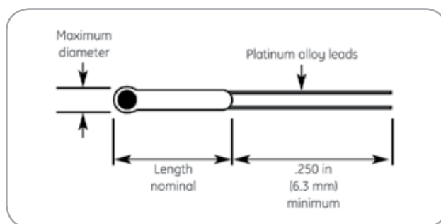
NTC Type HTP Series dimensions
