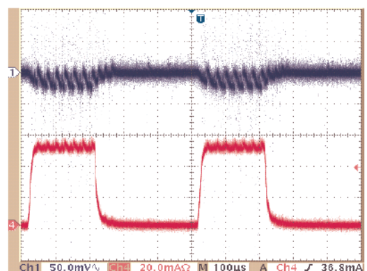
HT7727 Load Transient Response ( L=100\mu\text{H} , C_{\text{OUT}}=100\mu\text{F} , V_{\text{IN}}=1.62\text{V} )
