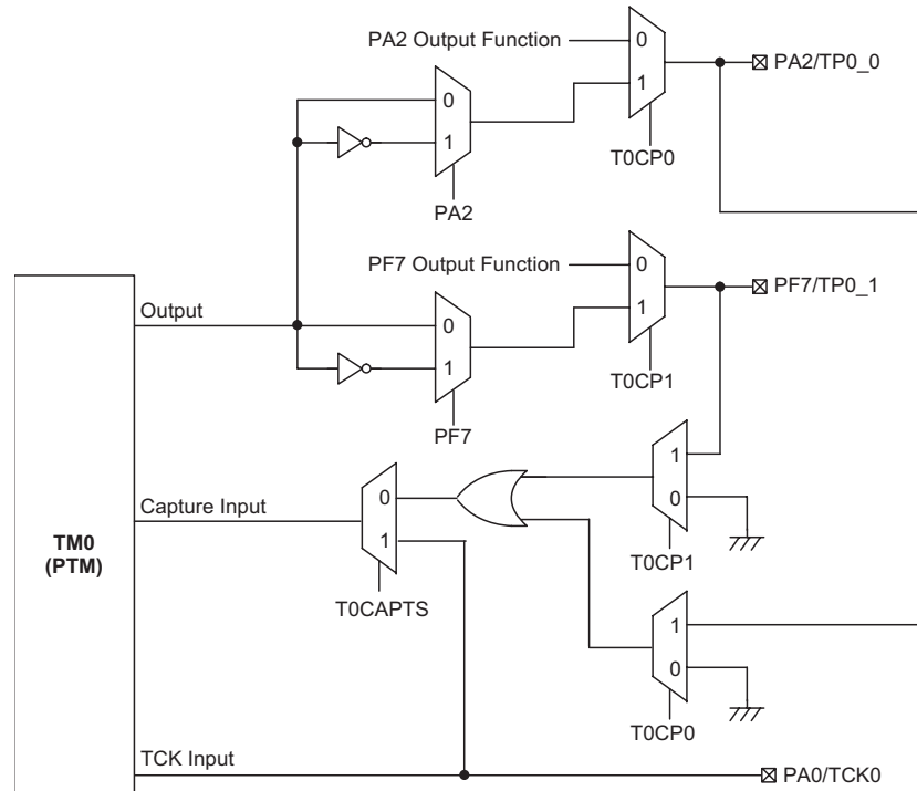
TM0 Function Pin Control Block Diagram
