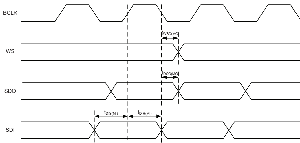
Figure 12. Timing of I²S Master Mode
