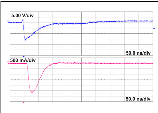
Figure 8. Response to ISO 7637-3 (pulse 3a) U_S = -150 V
