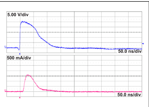
Figure 9. Response to ISO 7637-3 (pulse 3b) U_S = 100 V
