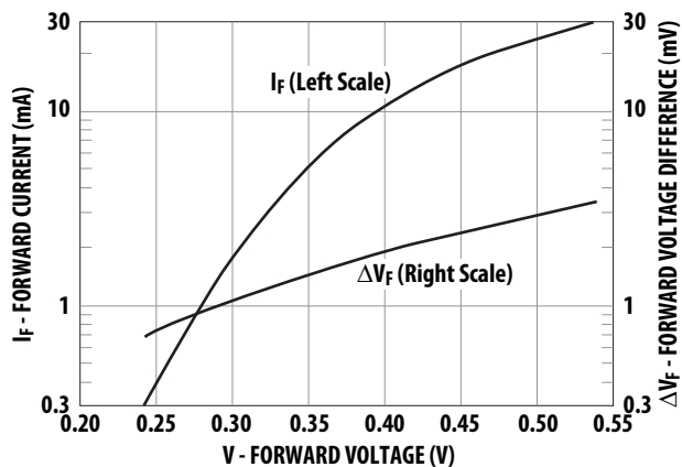
Figure 2. Typical VF Match, HSMS-820X Pairs and Quads.
