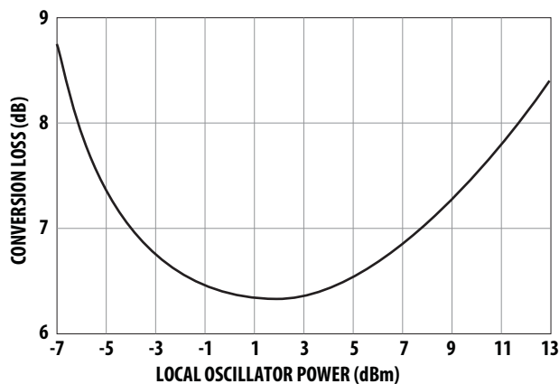
Figure 3. Typical Conversion Loss vs. Local Oscillator Power.
