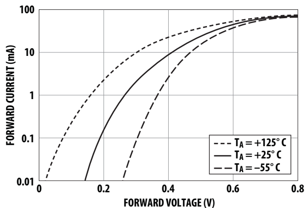
Figure 1. Typical Forward Current vs. Forward Voltage at Three Temperatures.
