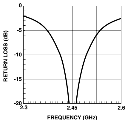
Figure 20. Input Return Loss. Modified 2.45 GHz Circuit.
