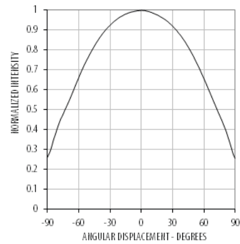
Figure 4 Radiation Pattern
