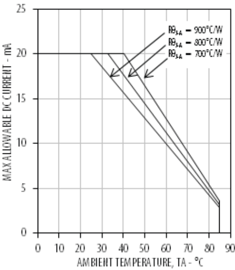
Figure 7 Derating Curve
