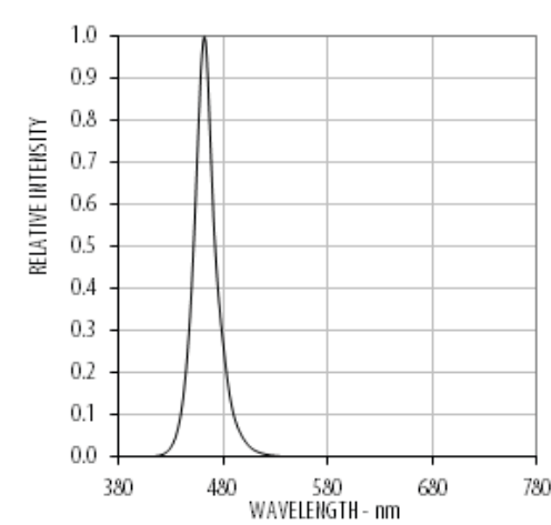
Figure 1 Spectrum
