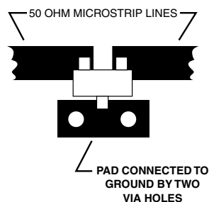
Figure 18. Circuit Layout.
