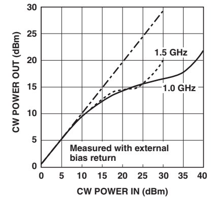
Figure 6. Large Signal Transfer Curve of the H5MP-482x Limiter.
