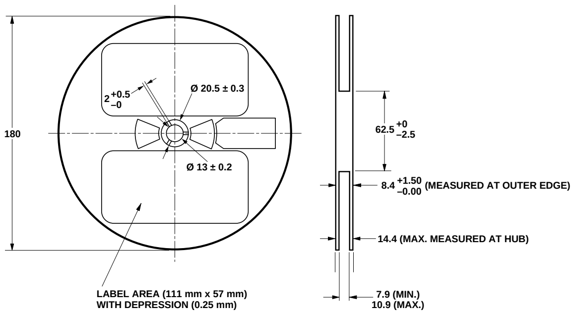
Figure 13. Reel dimensions.
