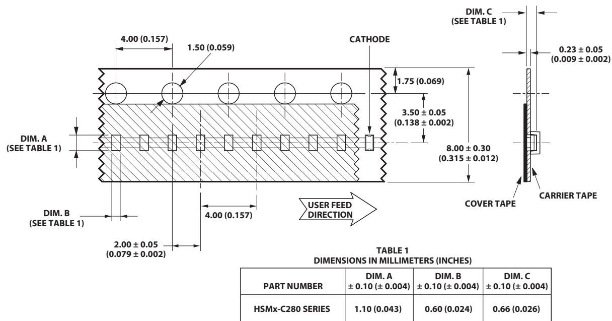
Figure 11. Tape dimensions.
