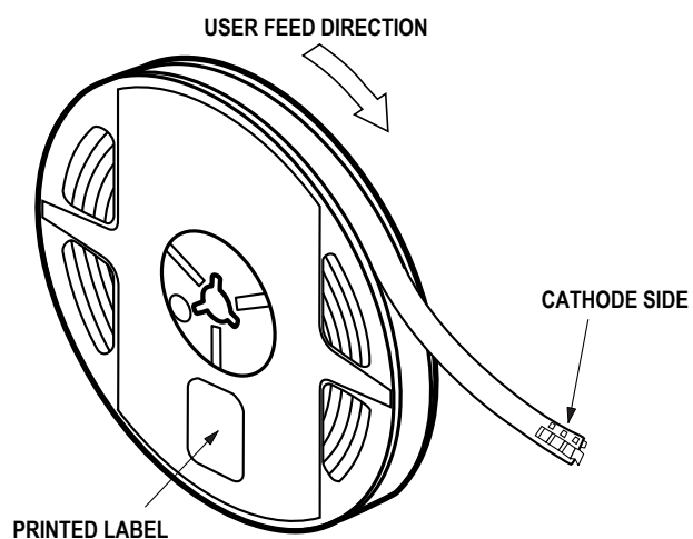
Figure 12. Reeling Orientation.
