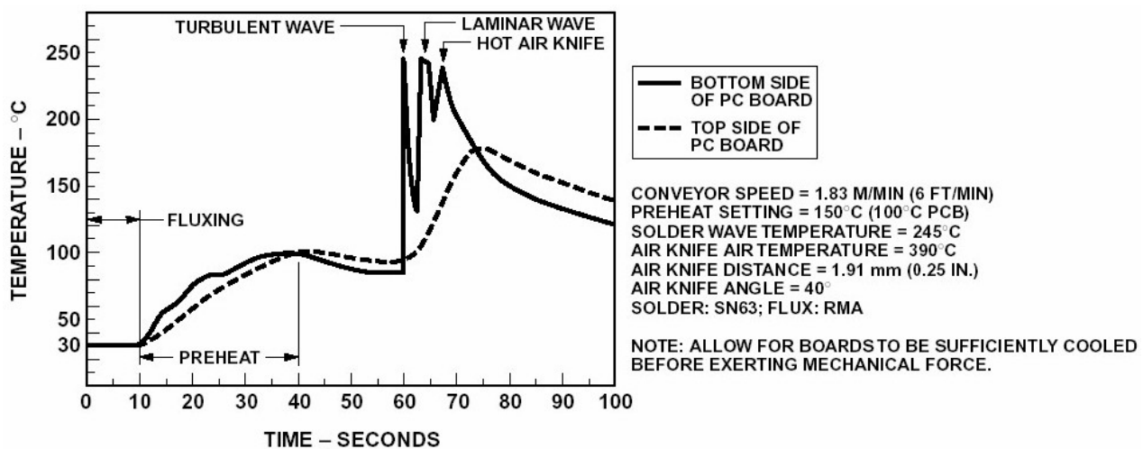
Figure 9. Recommended Wave Soldering Profile.
