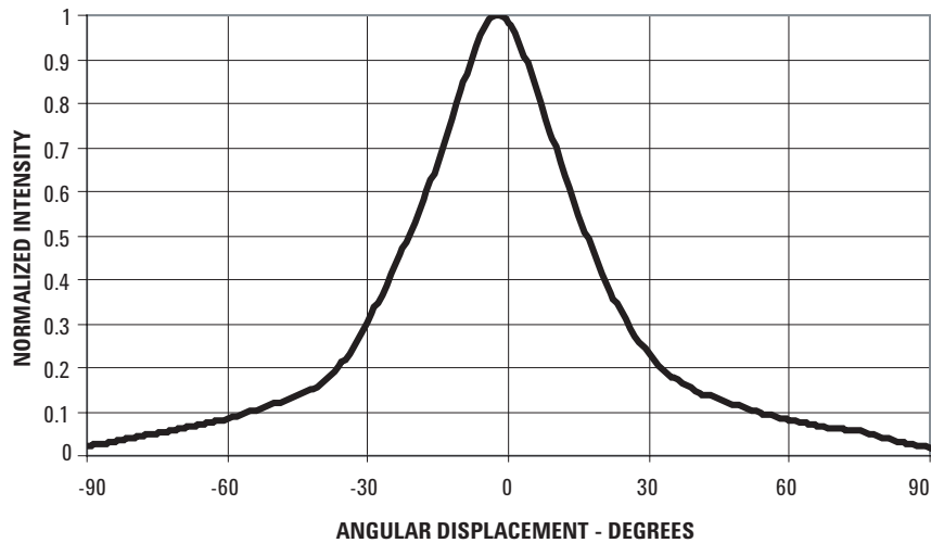
Figure 5. Radiation Pattern
