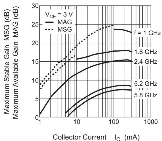
Maximum Stable Gain, Maximum Available Gain vs. Collector Current
