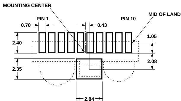
LAND PATTERN
