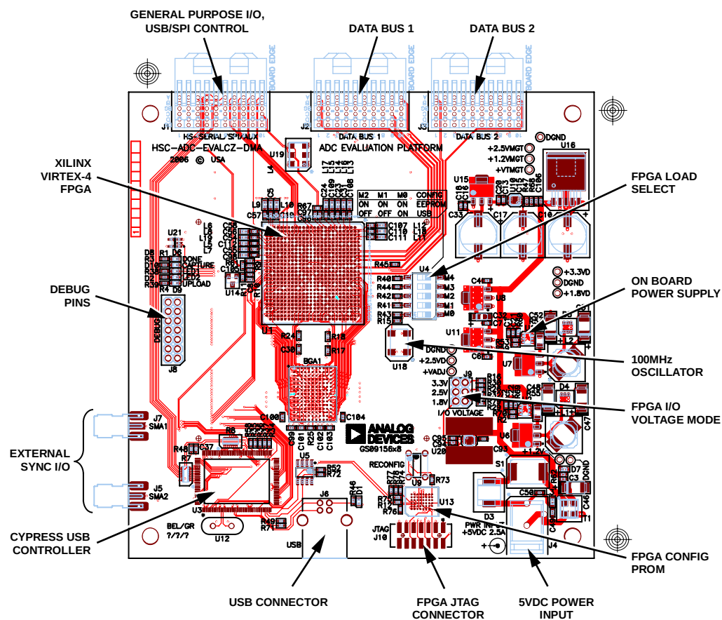
Figure 19. Top Silkscreen
