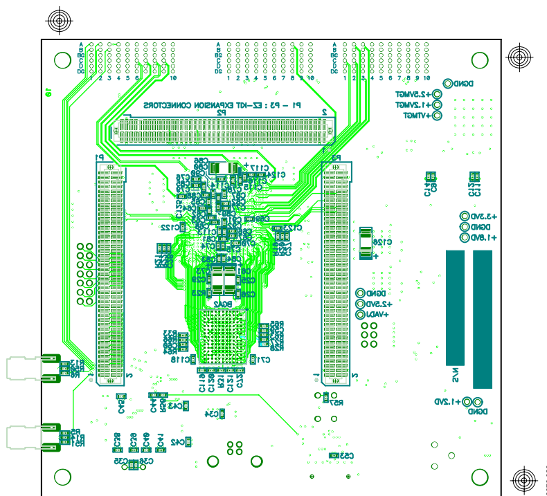
Figure 20. Bottom Silkscreen
