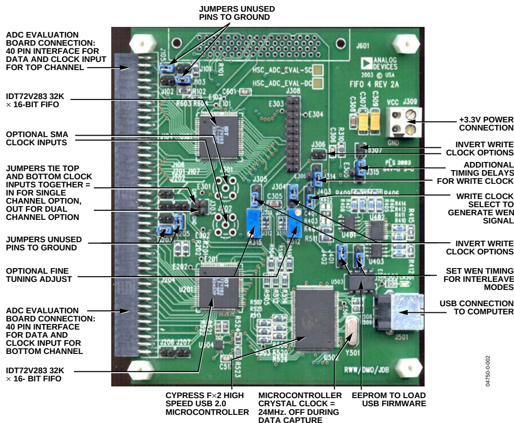
Figure 2. FIFO Components Description
