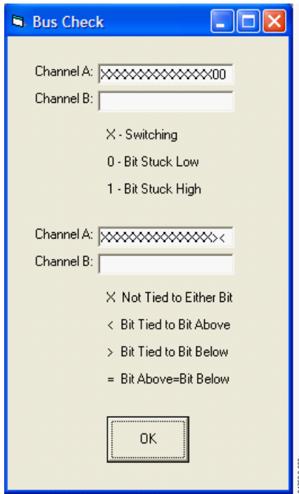
Figure 18. Bus Check for a 12-Bit ADC
