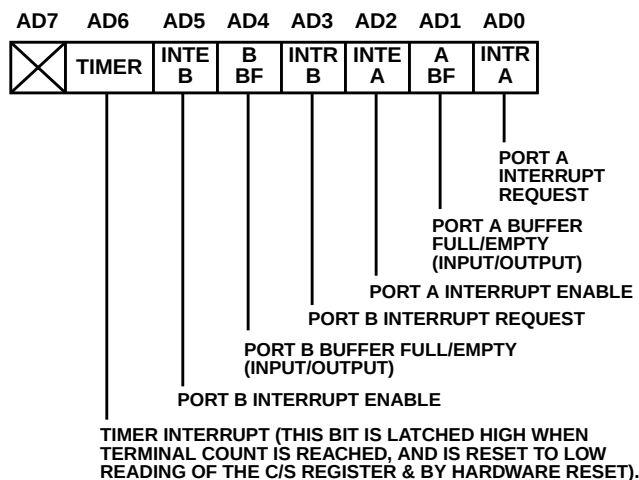
FIGURE 4. STATUS REGISTER BIT ASSIGNMENT
