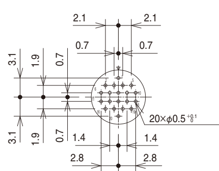
Size 9, 20 conductors
