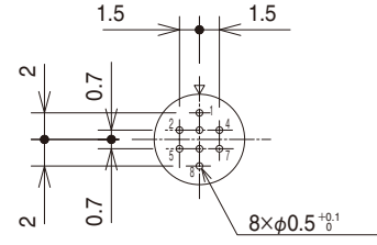
Size 7, 8 conductors
