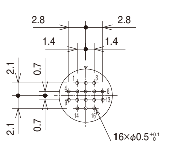
Size 9, 16 conductors
