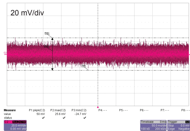
Figure 10: Output noise
