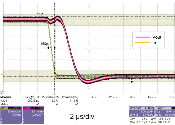
Figure 8: Step response
