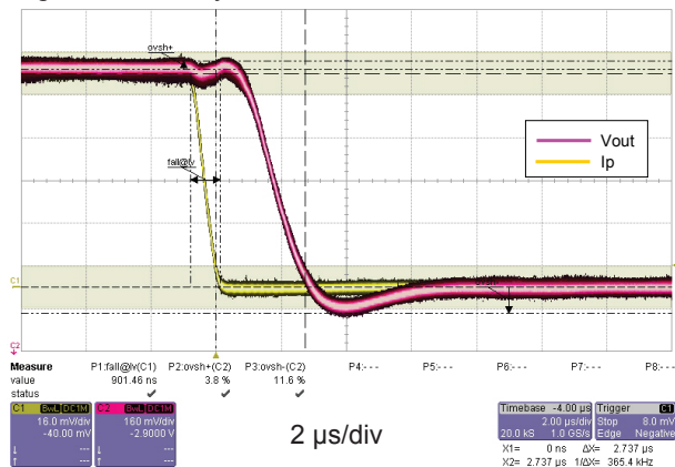
Figure 3: Step response
