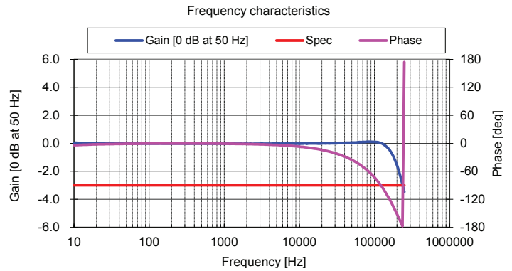
Figure 2: Frequency response
