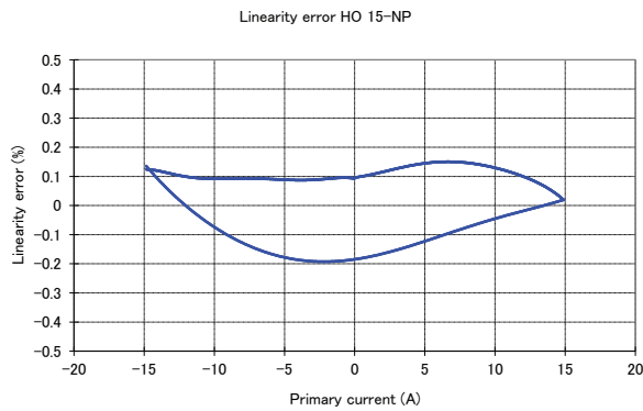
Figure 6: Linearity error
