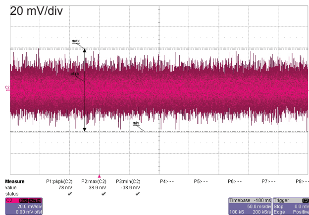
Figure 5: Output noise
