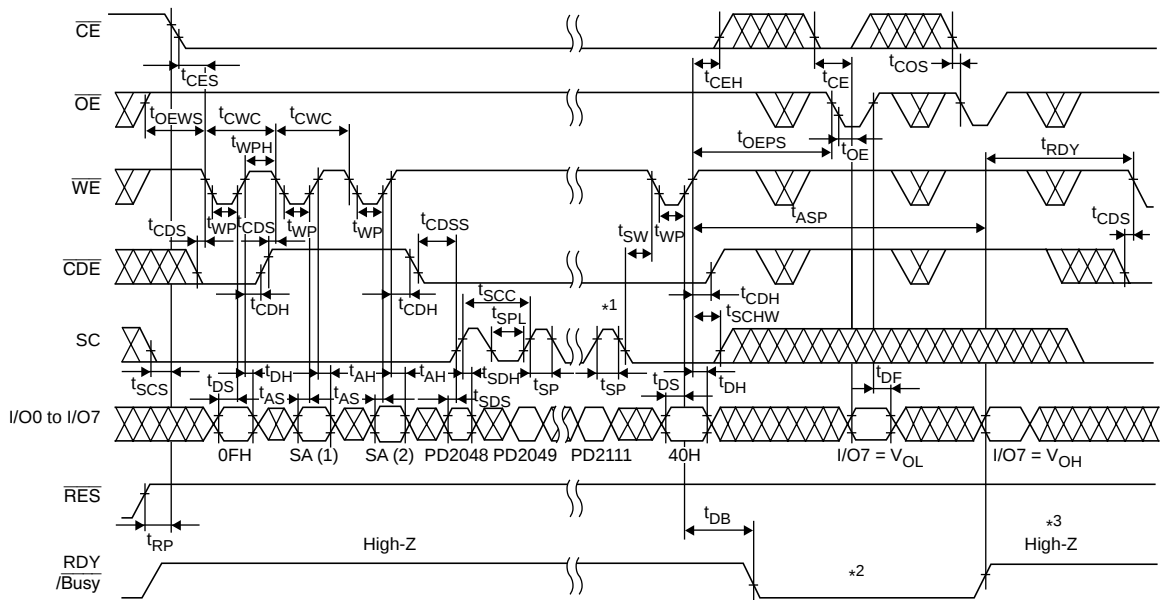
Program (3) and Status Data Polling Timing Waveform
