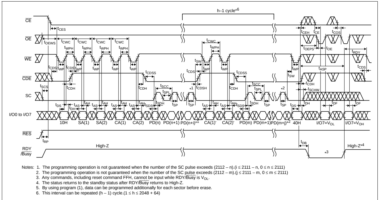
Program (1) with CA after SC and Status Data Polling Timing Waveform
