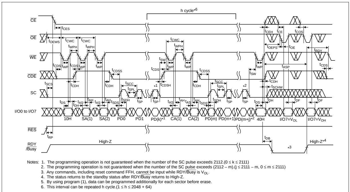
Program (1) with CA after SC and Status Data Polling Timing Waveform
