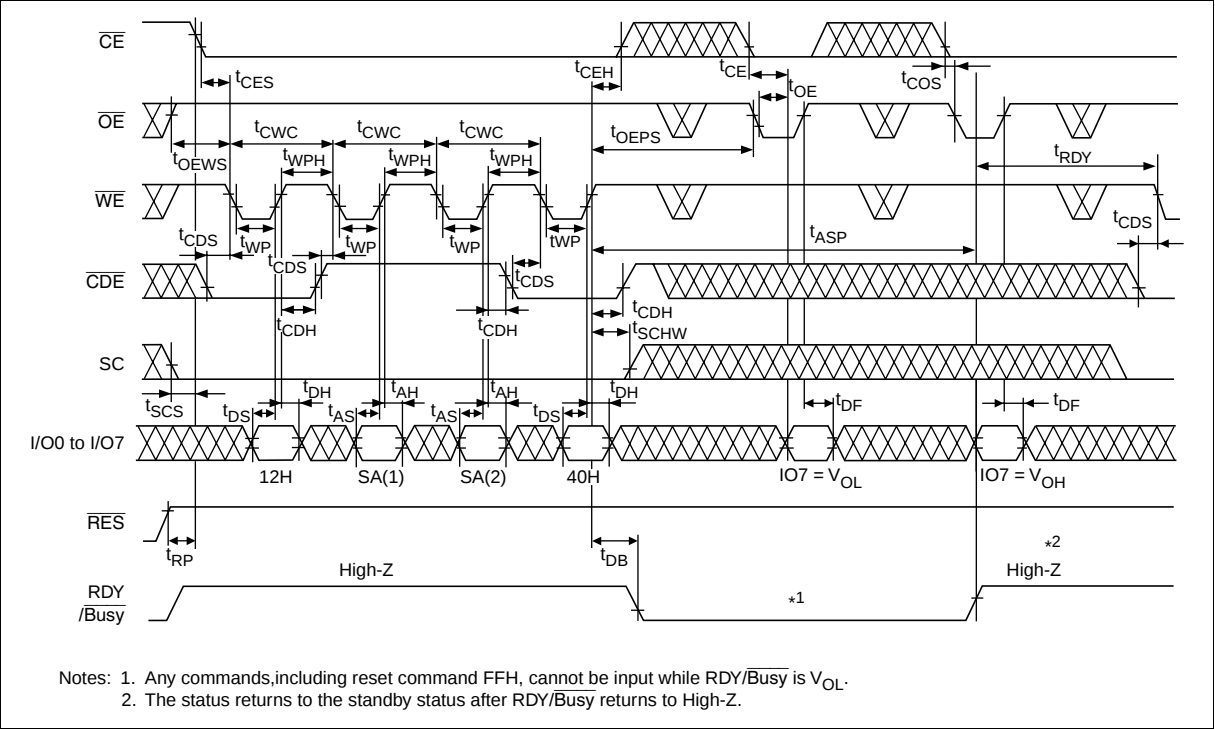
Data Recovery Write Timing Waveform
