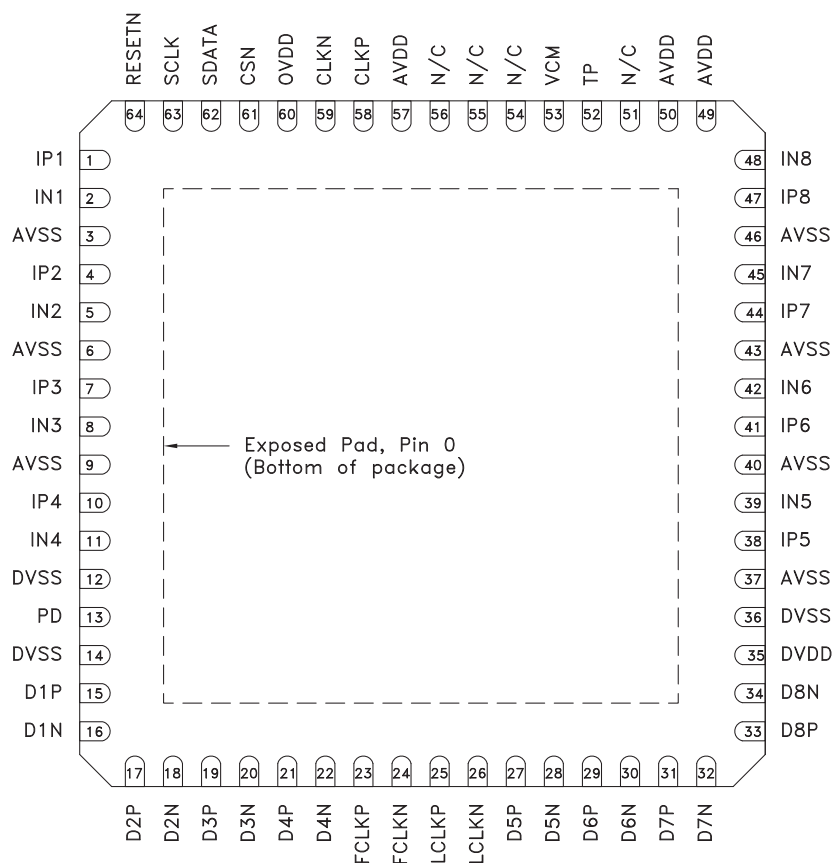
Figure 2. Package Diagram
