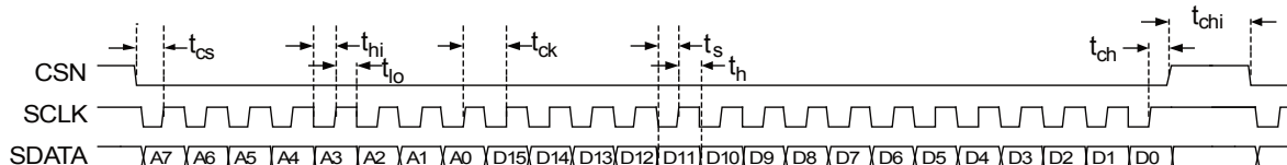
Figure 3. Serial Port Interface timing
