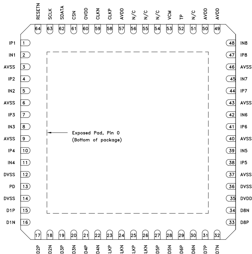
Figure 2. Package diagram
