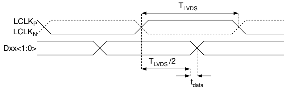
Figure 7. LVDS data timing, DDR mode
