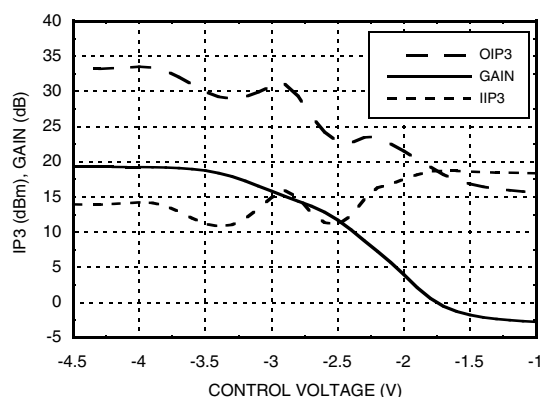
IP3 and Gain @ 6 GHz, P_{in} = -10 \text{ dBm}
