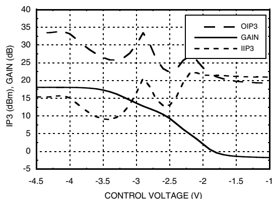
IP3 and Gain @ 10 GHz, P_{in} = -10 \text{ dBm}
