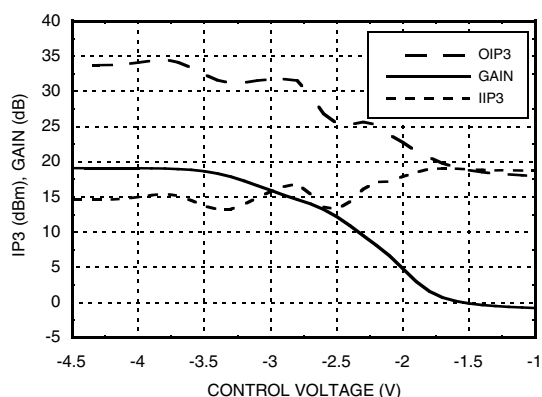
IP3 and Gain @ 8 GHz, P_{in} = -10 \text{ dBm}
