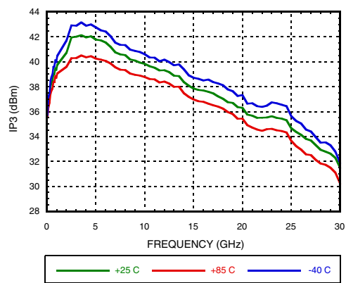
Output IP 3 vs. Temperature, P out /tone = +16 dBm
