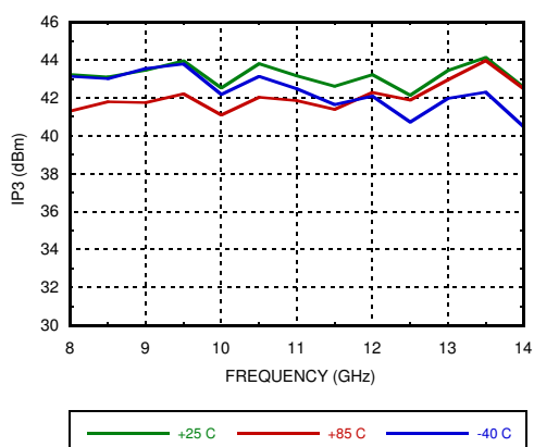
Output IP3 vs. Temperature, Pout/tone = +20 dBm
