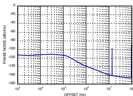
Figure 18. Fractional-N, Exact Frequency Mode OFF, Performance at 3591 MHz [8]
