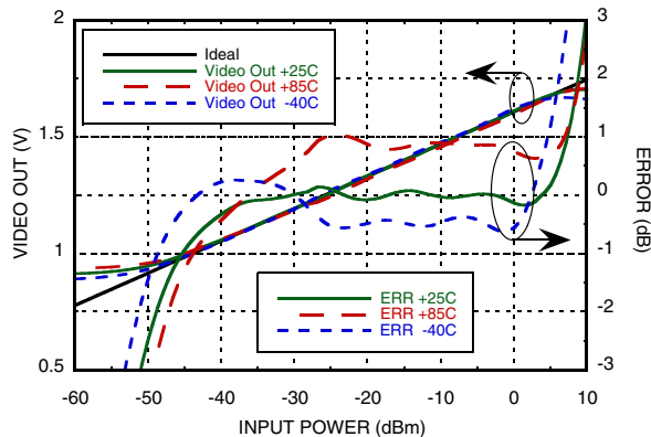
VIDEO OUT & Error vs. Input Power, f_{in} = 22\text{ GHz} [1]
