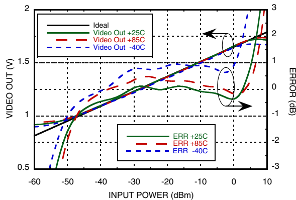
VIDEO OUT vs. Error vs. Input Power, f_{in} = 18\text{ GHz} [1]
