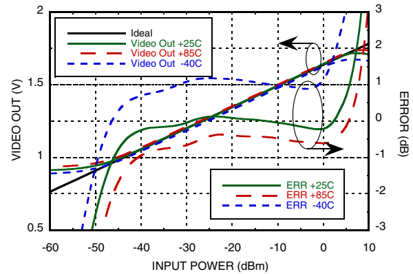
VIDEO OUT & Error vs. Input Power, f_{in} = 14\text{ GHz} [1]
