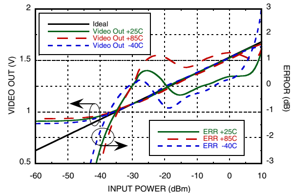
VIDEO OUT & Error vs. Input Power, f_{in} = 26\text{ GHz} [1]
