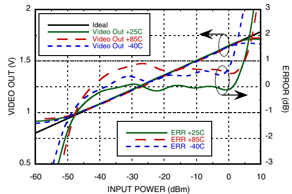
VIDEO OUT & Error vs. Input Power, f_{in} = 20\text{ GHz} [1]
