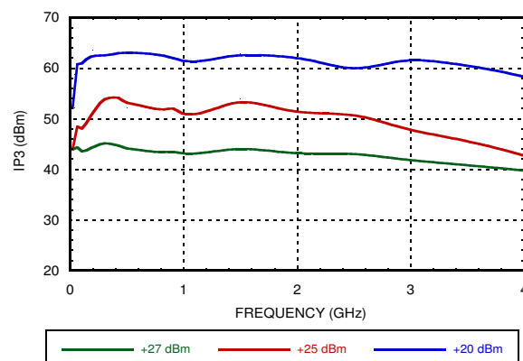
Input IP3 vs. Tone Power @ Vdd = +3V
