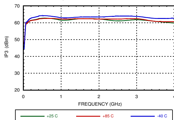
Input IP3 vs. Temperature 27 dBm Tones, Vdd = +5V
