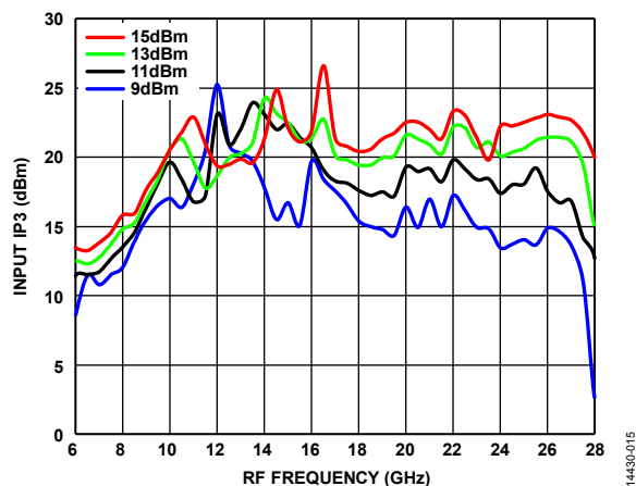
Figure 16. Input IP3 vs. RF Frequency at Various LO Drives
