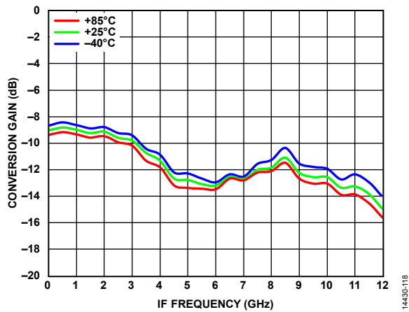
Figure 18. Conversion Gain vs. IF Frequency at Various Temperatures
