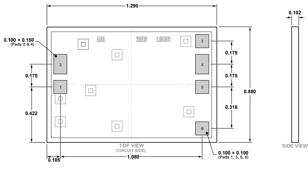
Figure 67. 6-Pad Bare Die [CHIP] (C-6-12) Dimensions shown in millimeter
