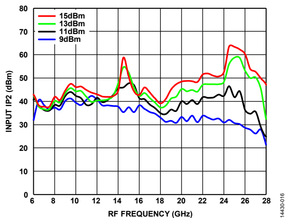
Figure 17. Input IP2 vs. RF Frequency at Various LO Drives
