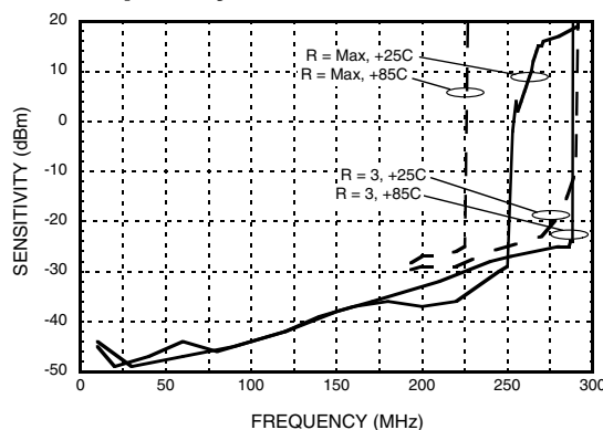
Typical Reference Sensitivity vs. Frequency, 3.3V [1]
