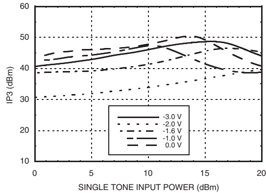
Input IP3 vs Input Power @ 10 GHz V_{ctrl1} = \text{Variable} , V_{ctrl2} = -3V
