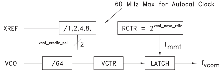
Figure 18. VCO Calibration
