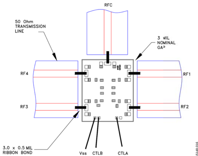
Figure 16. Die Assembly Diagram
