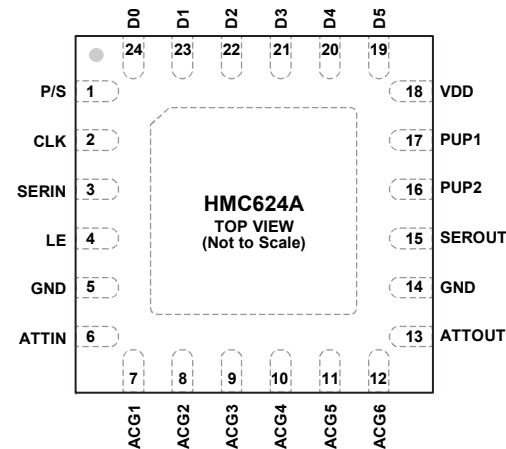
Figure 3. Pin Configuration
