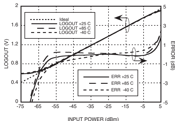
LOGOUT Voltage & Error vs. Input Power, f_{in} = 900 MHz
