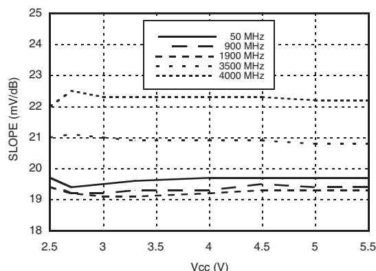
LOGOUT Slope vs. Supply Voltage, T A = +25°C
